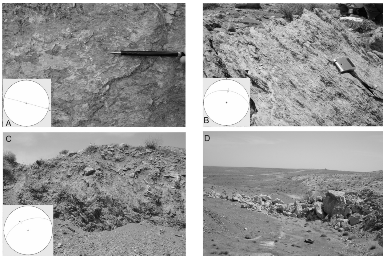
Figure 4. Samples of fault types in the study area. A) A left lateral strike-slip fault in central Laibid, B) North dipping thrust zone in western Laibid, C and D) North dipping normal fault zone in northern boundary of western Laibid.
