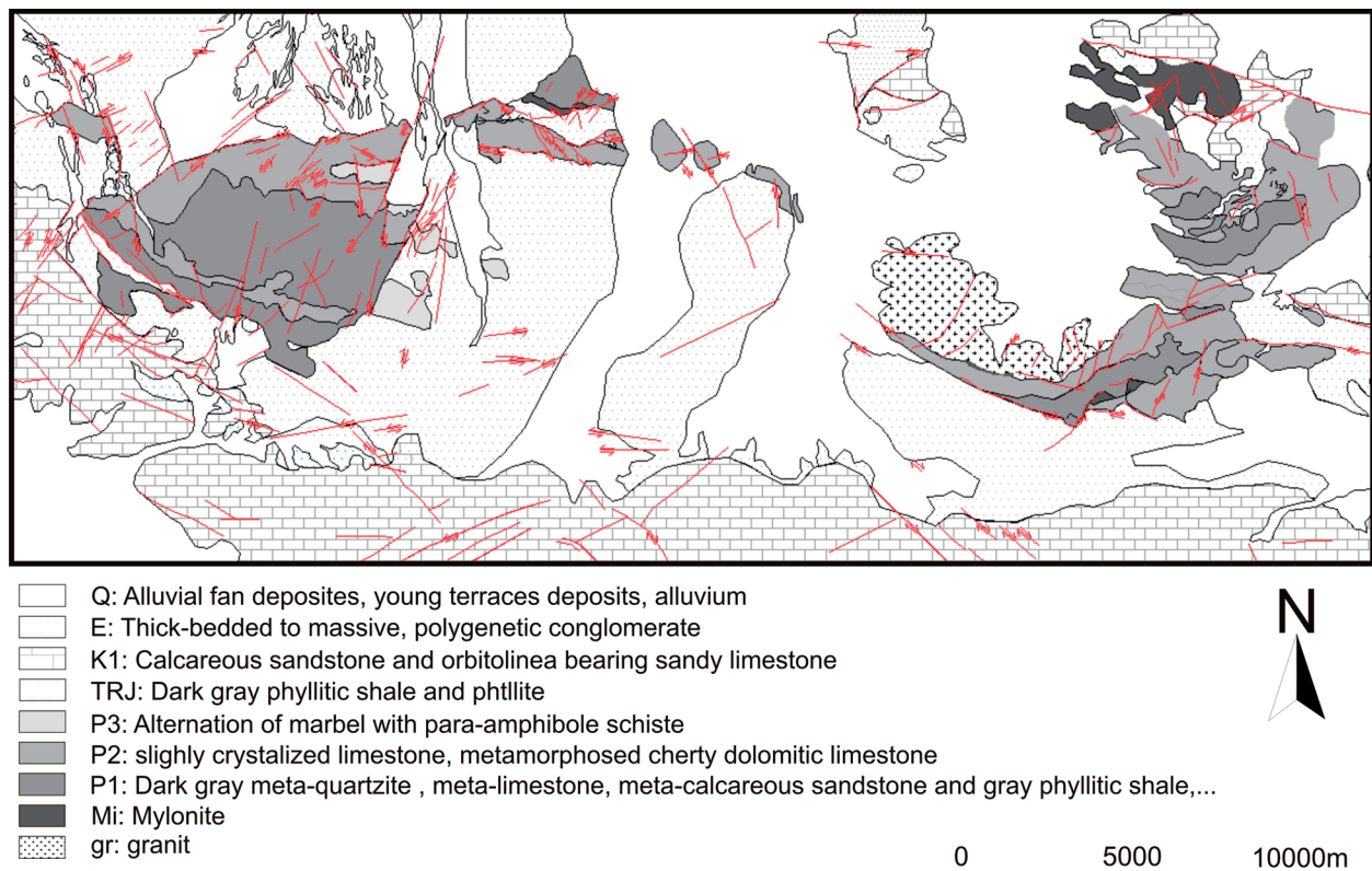
Figure 2. Geological map of Laibid pop-up structure.
