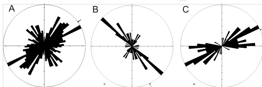
Figure 5. Rose diagrams of the total (A), right-lateral (B) and left-lateral (C) fault trends in Laibid area.
