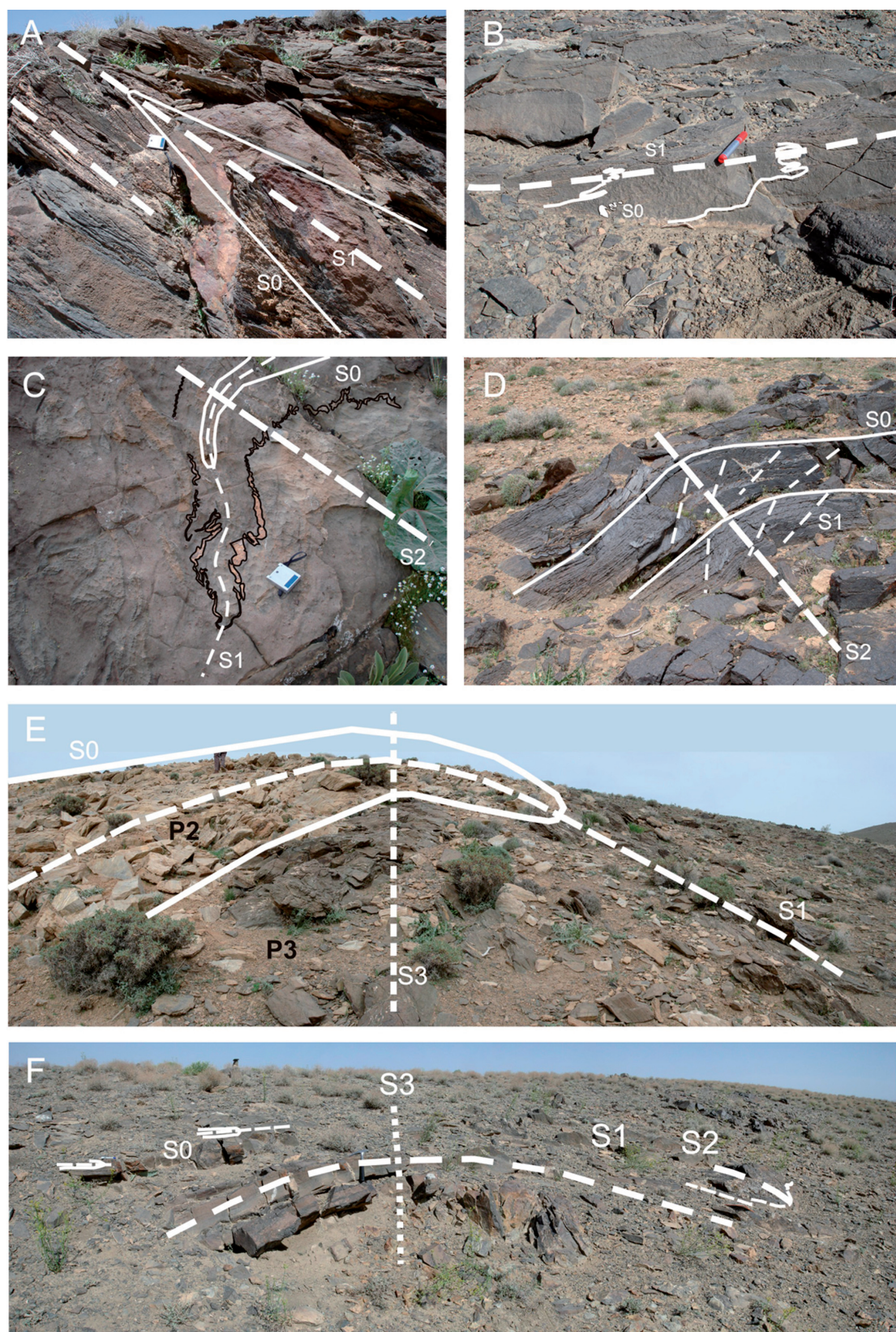
Figure 3. Samples reveal the folding style in the first (A and B), second (C and D) and third (E and F) stage and coaxial interference patterns resulting from folding stage superposition.
